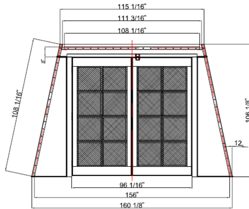
END VIEW FROM BAY END
