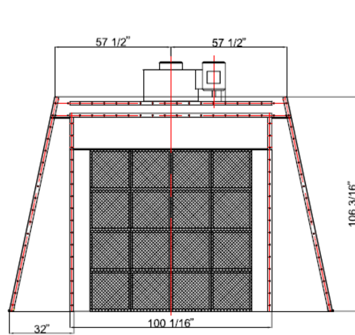
END VIEW @ CHAMBER
