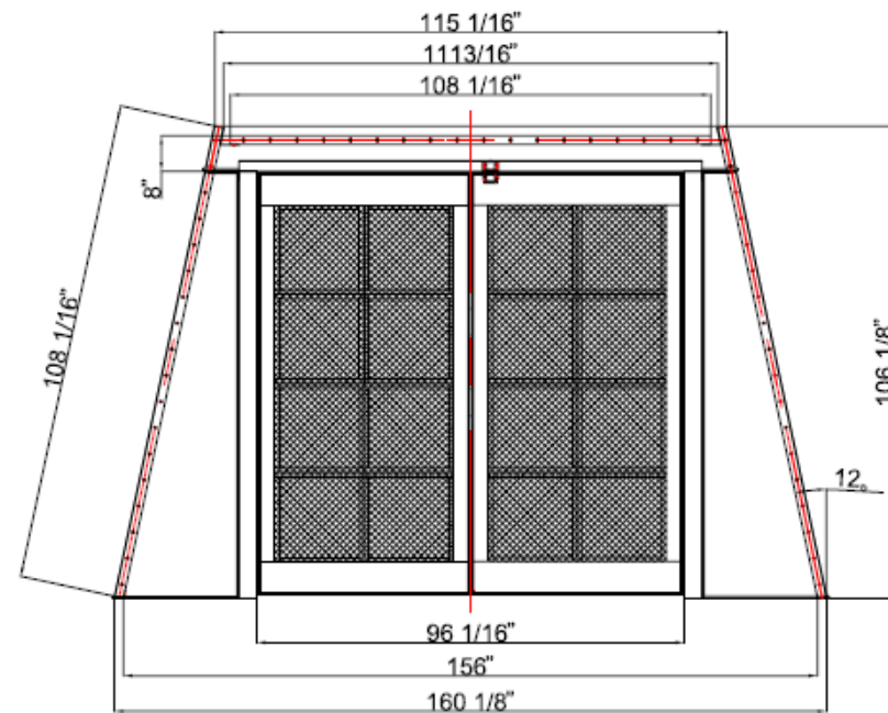
END VIEW FROM BAY END
