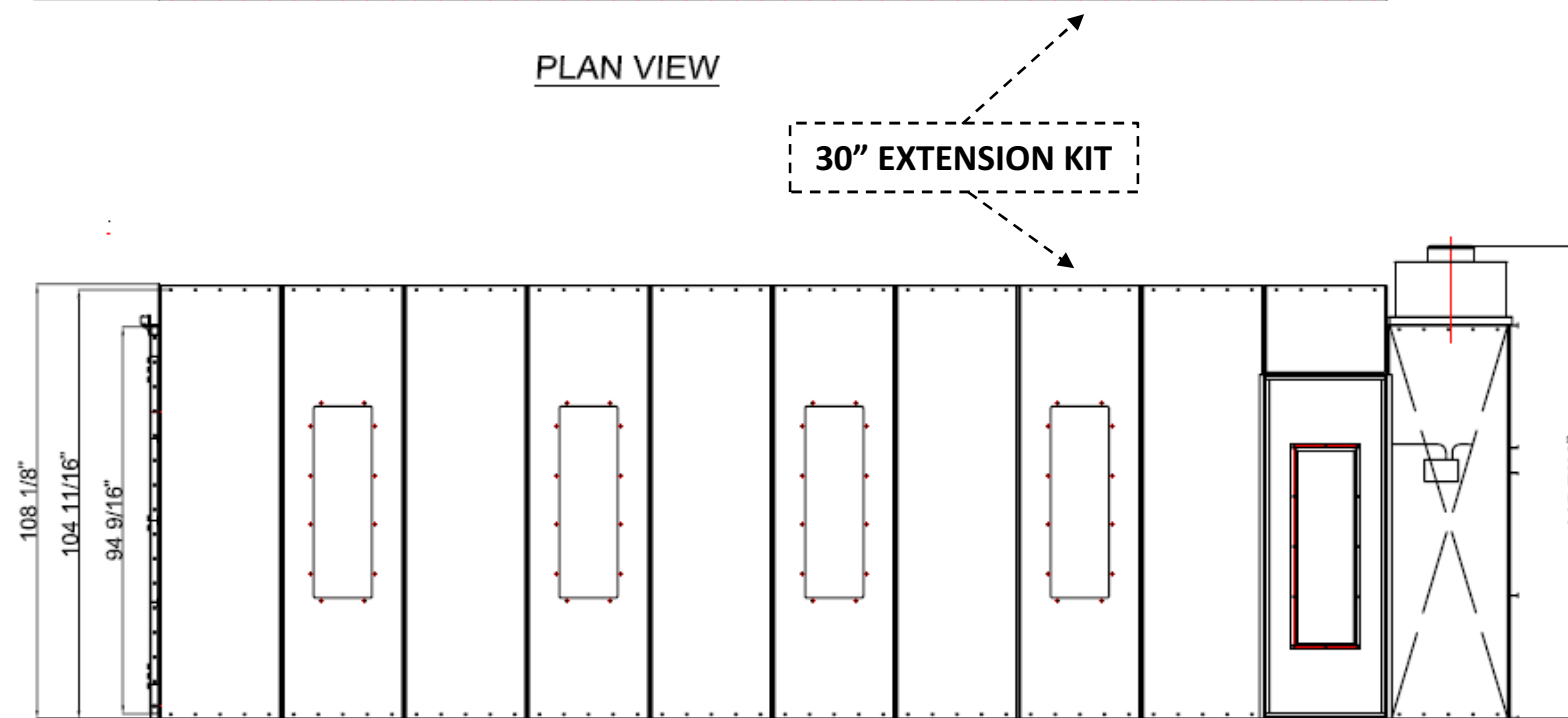
BOOTH SIDE VIEW
